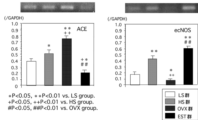
Fig. 10. Expression of angiotensin converting enzyme (ACE) -mRNA (left panel) and endothelium constitutive Nitric Oxide synthase (ecNOS) -mRNA in the heart in Dahl salt sensitive (Dahl-S) rats with myocardial infarction. Open bar indicates low-salt (LS) group, small dot bar indicates high-salt (HS) group, large dot bar indicates ovariectomy (OVX) group and closed bar indicates estrogen treated (EST) group. Values are means \pm SEM. *P<0.05, **P<0.01 vs. LS group. +P<0.05, ++P<0.01 vs. HS group, and #P<0.05, ##P<0.01 vs. OVX group.
